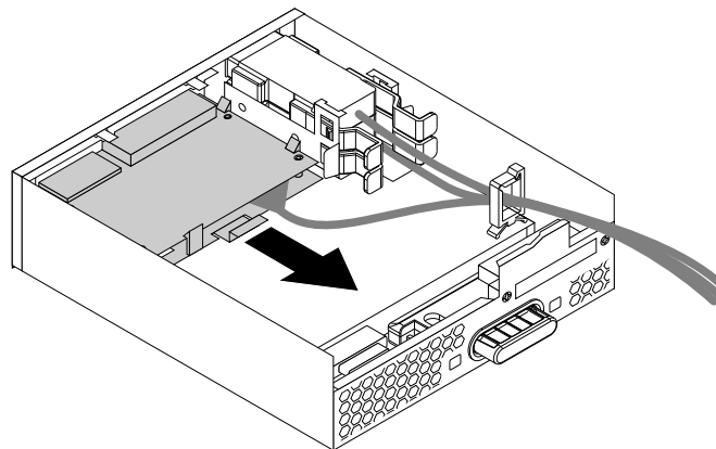
Figure 86. Removing the card reader in the flex module
