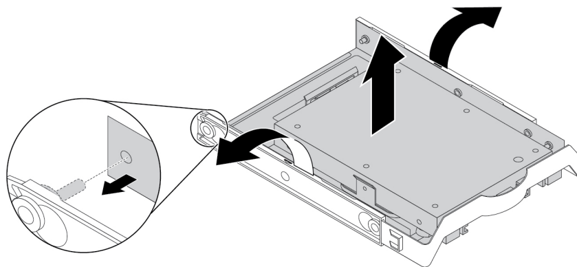
Figure 125. Removing the storage converter from the 3.5-inch storage drive bracket
