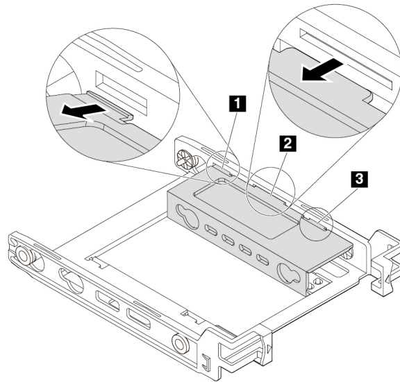
Figure 71. Releasing tabs 1 , 2 , and 3 from the corresponding slots
