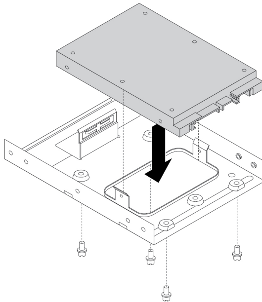
Figure 127. Installing the new solid-state drive into the storage converter
