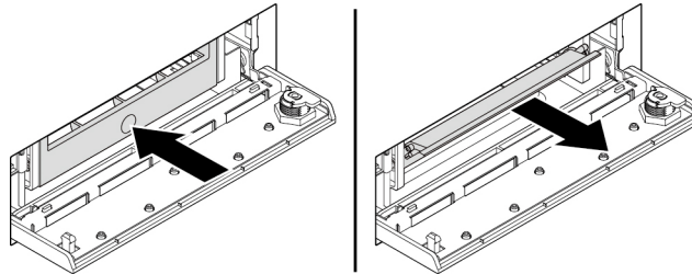
Figure 41. Removing the bracket from the front-access storage enclosure
