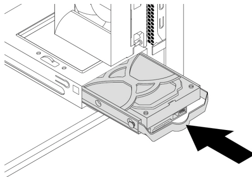
Figure 122. Installing the secondary hard disk drive
