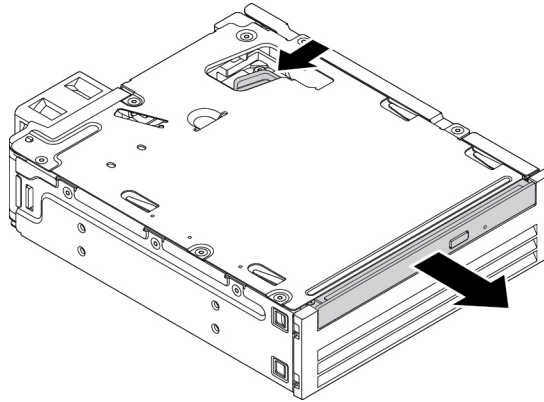
Figure 50. Removing the slim optical drive from the kit
