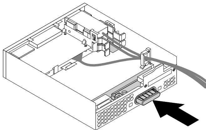
Figure 76. Removing the slim optical drive from the flex module
