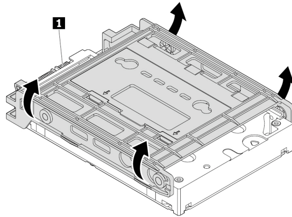
Figure 56. Flexing both sides of the bracket to remove the 3.5-inch internal storage drive
