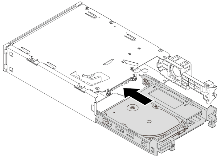
Figure 64. Sliding the new 2.5-inch internal storage drive into the kit
