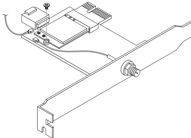
Figure 145. Installing a screw to secure the Wi-Fi card module
