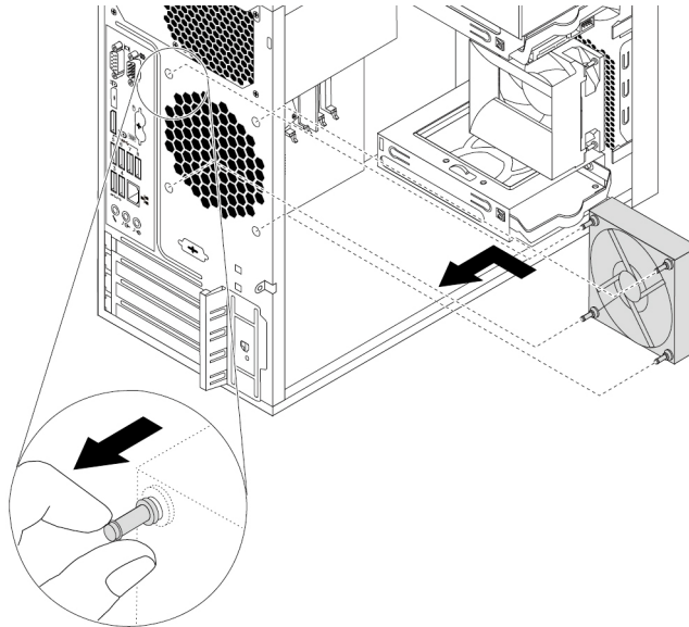
Figure 132. Installing the rear fan assembly
