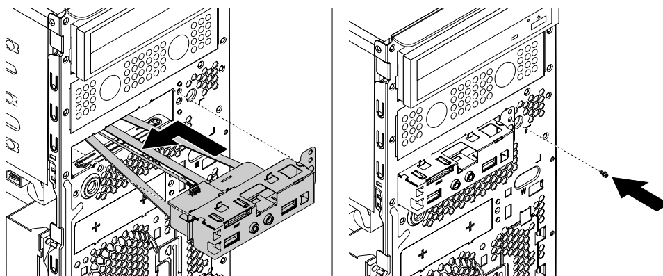
Figure 102. Installing the front audio and USB assembly
