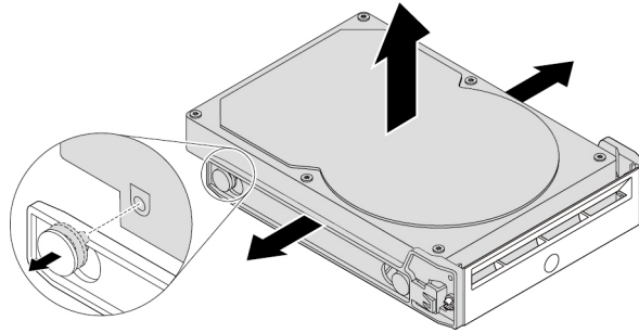
Figure 37. Removing the 3.5-inch storage drive from the bracket
