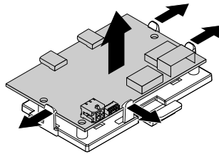
Figure 93. Removing the front Thunderbolt I/O adapter from the retaining bracket
