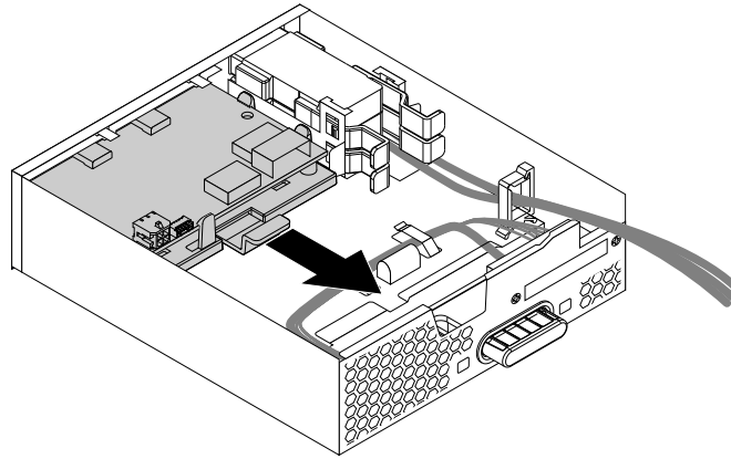
Figure 92. Removing the front Thunderbolt adapter and the retaining bracket out of the flex module
