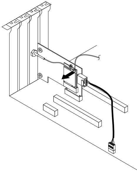
Figure 133. Disconnecting the front Wi-Fi antenna cable
