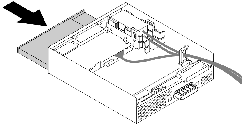
Figure 79. Installing the slim optical drive in the flex module
