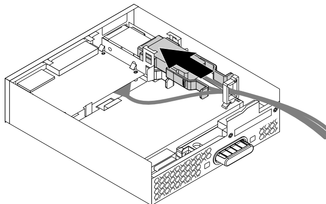
Figure 83. Installing the eSATA connector or IEEE 1394 connector in the flex module
