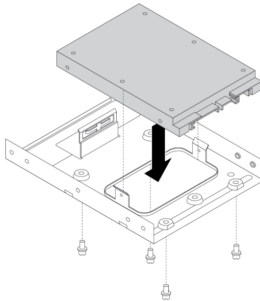
Figure 123. Installing the solid-state drive into the storage converter
