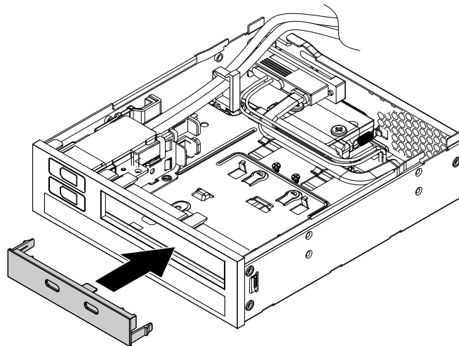
Figure 94. Installing the bezel to the flex module
