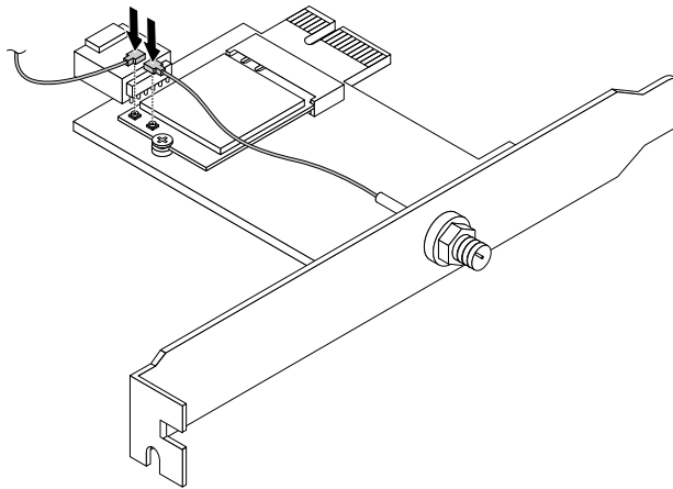
Figure 146. Installing the Wi-Fi antenna cables
