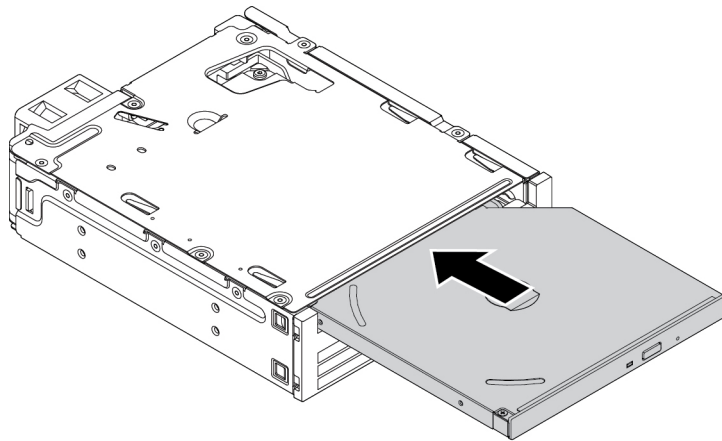
Figure 53. Installing the slim optical drive into the kit
