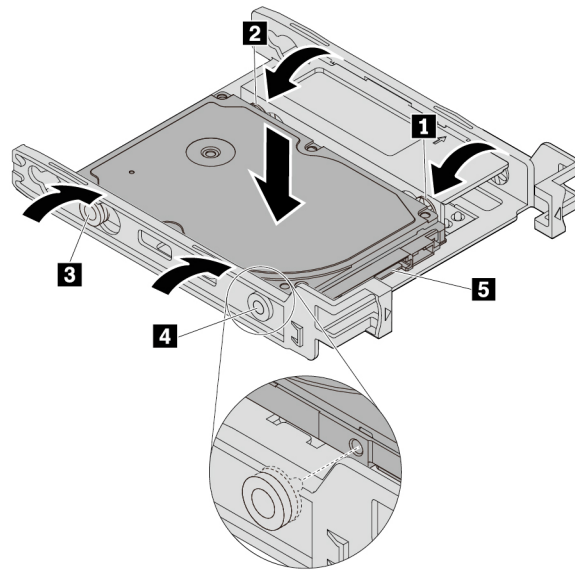
Figure 63. Installing the new 2.5-inch internal storage drive into the bracket
