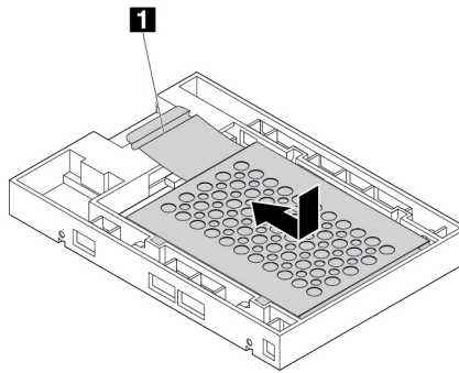
Figure 47. Installing the metal bracket into the plastic frame of the converter
