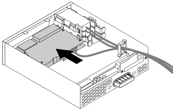
Figure 89. Installing the card reader in the flex module
