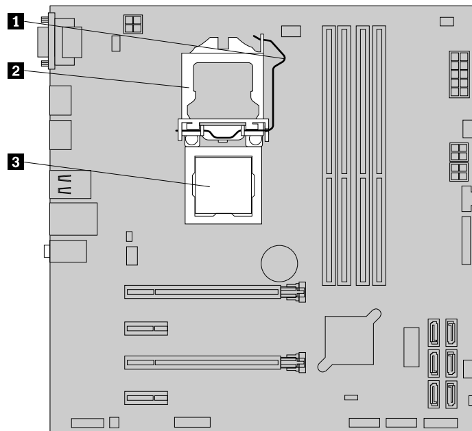
Figure 111. Accessing the microprocessor
