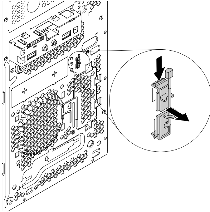
Figure 105. Removing the thermal sensor
