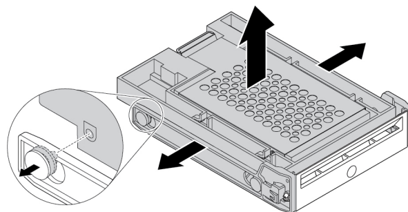
Figure 42. Removing the 2.5-inch storage drive from the bracket
