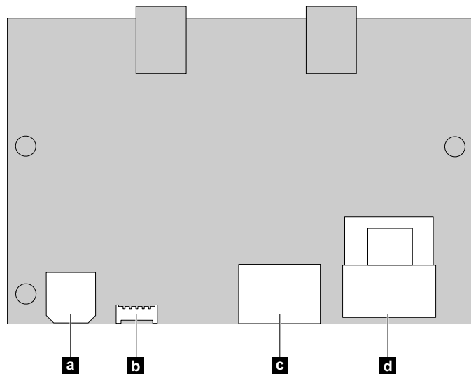
Figure 97. Front Thunderbolt adapter cable connection
