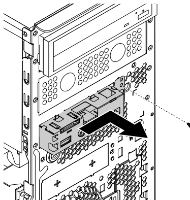
Figure 101. Removing the front audio and USB assembly
