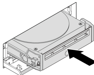
Figure 39. Installing the 3.5-inch storage drive into the front-access storage enclosure
