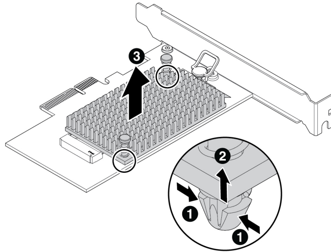
Figure 21. Removing the heat sink from the M.2 solid-state drive adapter
