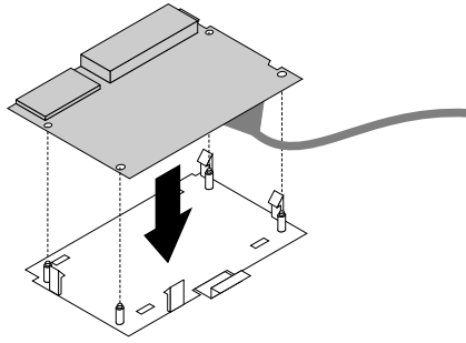
Figure 88. Installing the card reader into the card-reader retaining bracket
