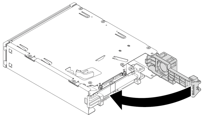
Figure 59. Pivoting the rear cover inward
