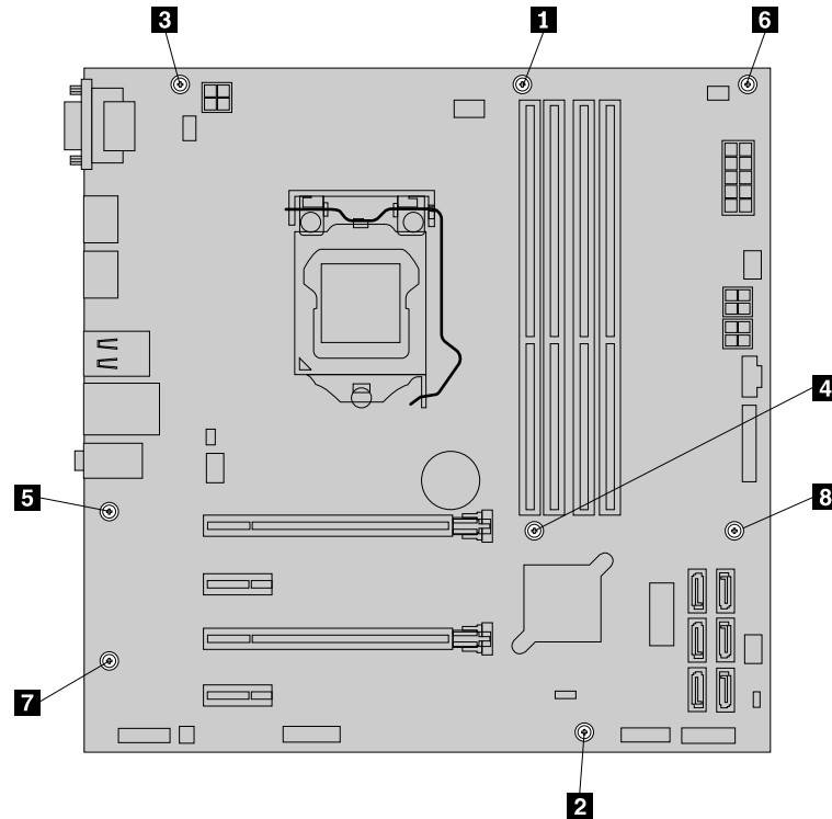
Figure 115. Installing the eight screws to secure the system board
