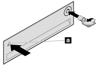
Figure 40. Opening the front-access storage enclosure cover
