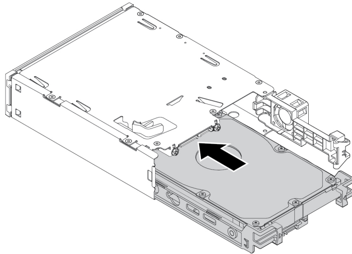
Figure 58. Sliding the new 3.5-inch internal storage drive into the kit
