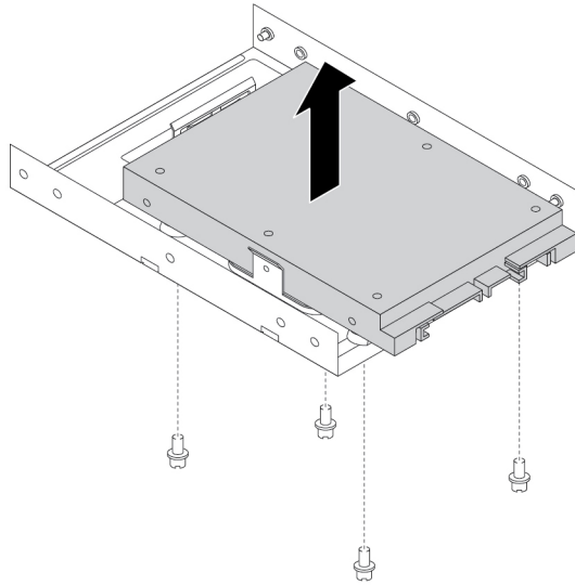
Figure 126. Removing the solid-state drive from the storage converter
