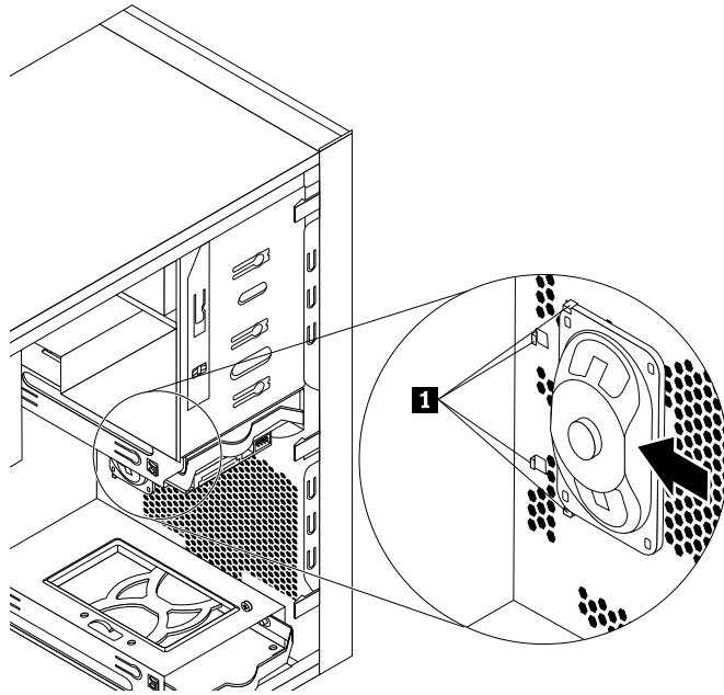
Figure 104. Installing the internal speaker
