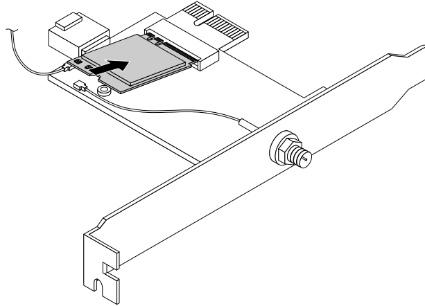
Figure 144. Installing the Wi-Fi card module
