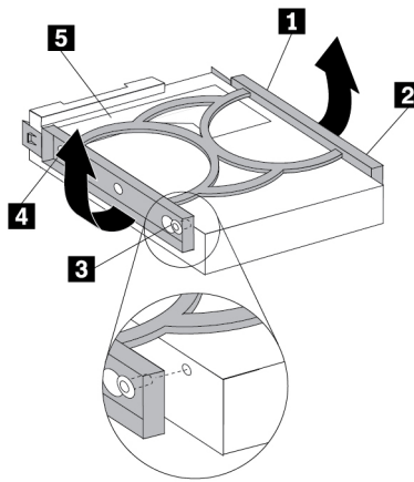
Figure 121. Installing the hard disk drive into the bracket
