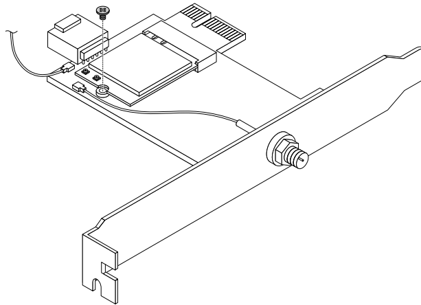
Figure 140. Removing the screw that secures the Wi-Fi card module
