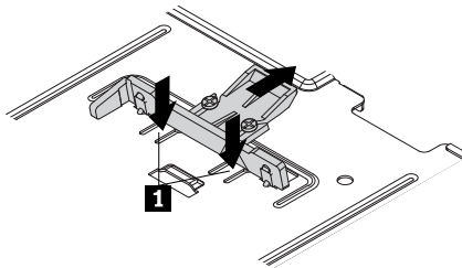
Figure 75. Removing the plastic clip with the two screws
