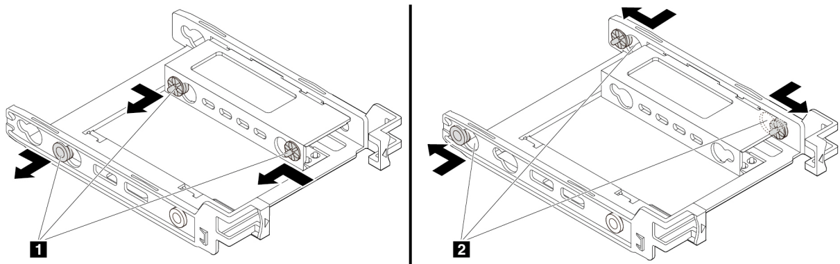
Figure 70. Removing three pins 1 and installing them into slots 2
