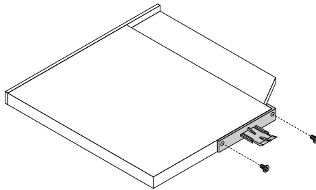
Figure 78. Installing the plastic clip to the slim optical drive
