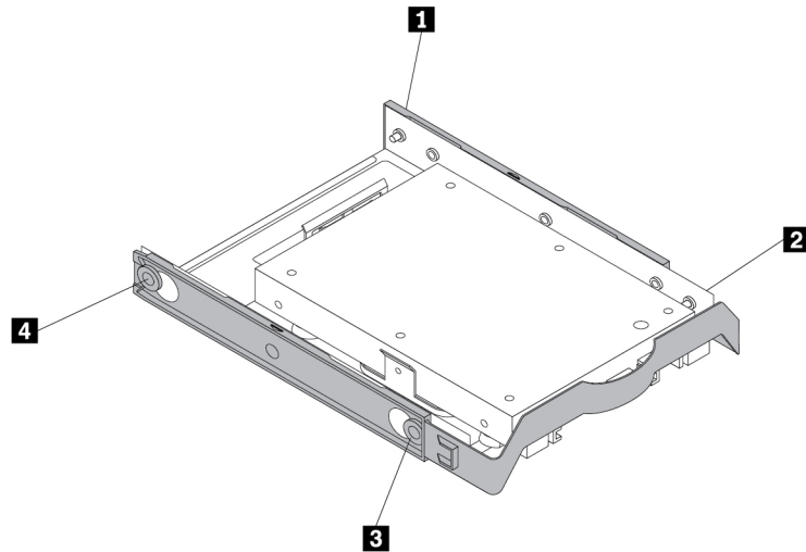
Figure 128. Installing the storage converter with the new solid-state drive into the storage drive bracket
