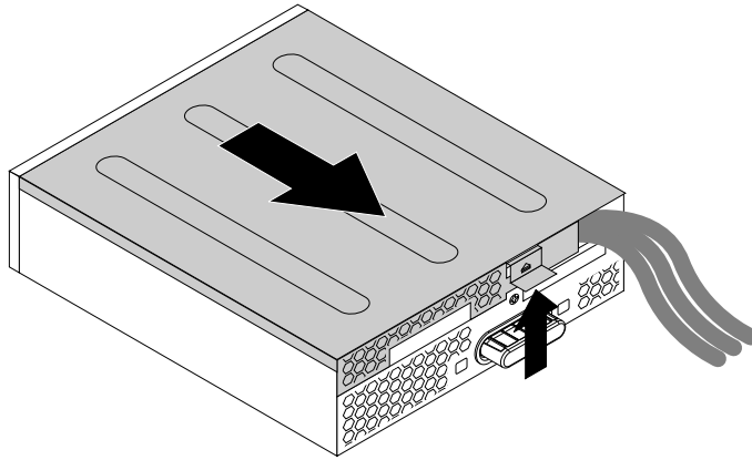
Figure 74. Removing the flex module cover
