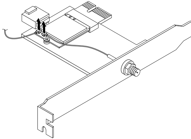
Figure 139. Disconnecting the Wi-Fi antenna cables
