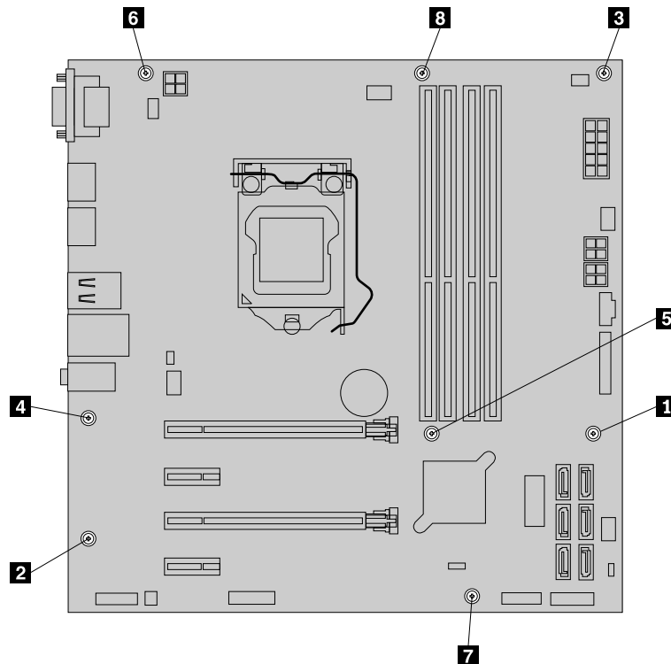
Figure 114. Removing the eight screws that secure the system board
