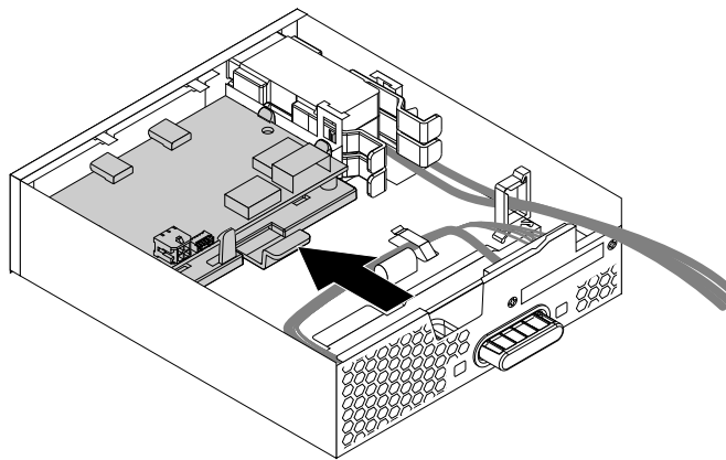
Figure 96. Installing the front Thunderbolt adapter and the retaining bracket into the flex module
