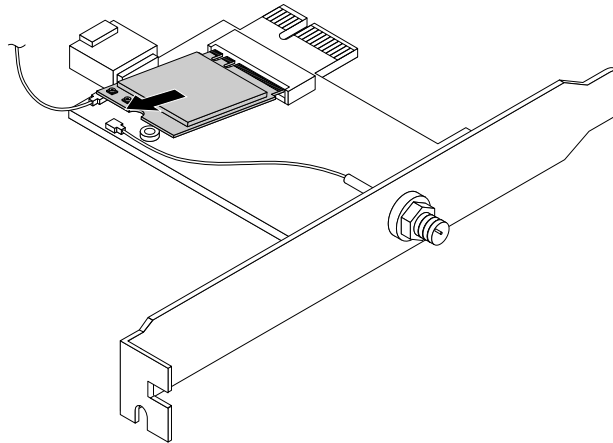
Figure 141. Removing the Wi-Fi card module
