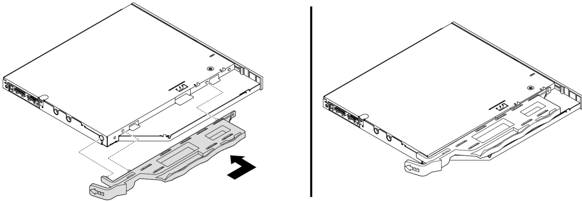
Figure 52. Installing the bracket to the new slim optical drive
