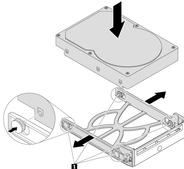
Figure 38. Installing the 3.5-inch storage drive into the bracket
