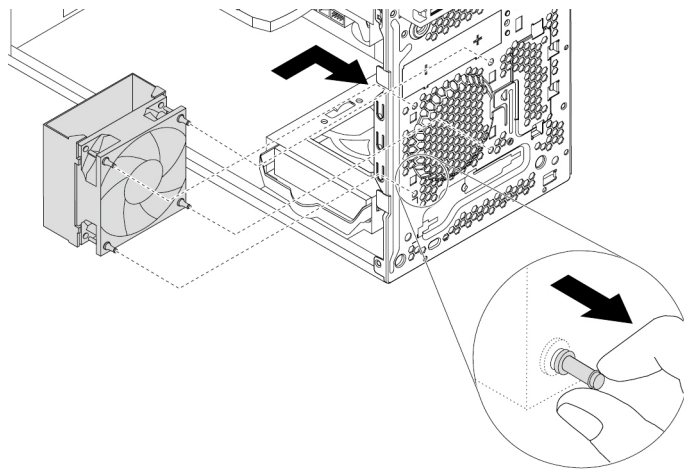
Figure 130. Installing the front fan assembly
