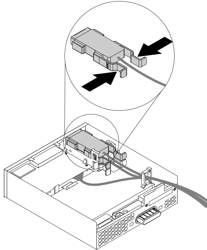
Figure 82. Removing the eSATA connector or IEEE 1394 connector in the flex module
