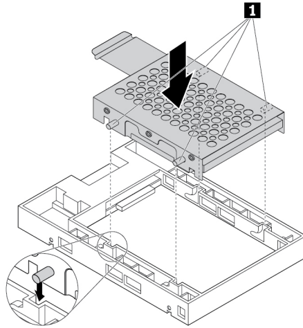
Figure 46. Inserting the metal bracket into the plastic frame of the converter
