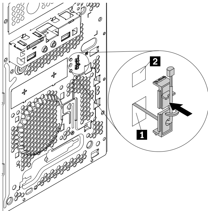
Figure 106. Installing the thermal sensor
