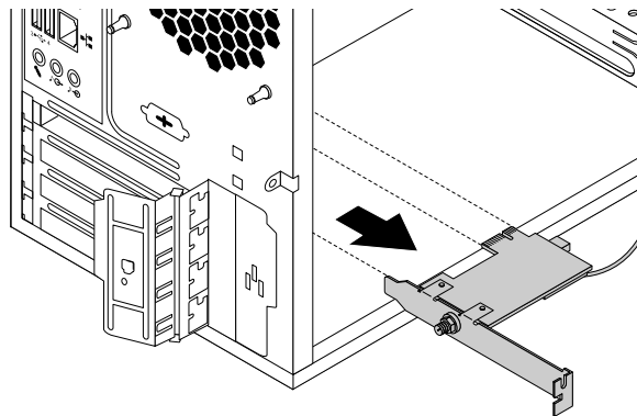
Figure 138. Removing the Wi-Fi adapter card
