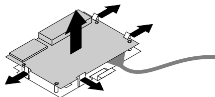
Figure 87. Removing the card reader from the card-reader retaining bracket
