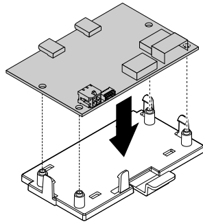
Figure 95. Installing the front Thunderbolt I/O adapter into the retaining bracket
