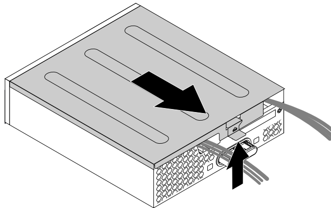
Figure 91. Removing the flex module cover
