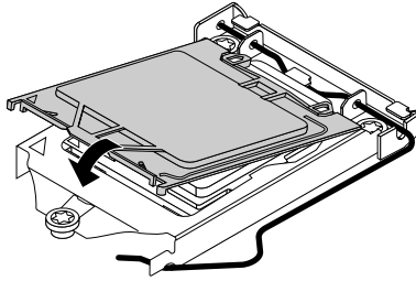
Figure 116. Installing the microprocessor socket cover
