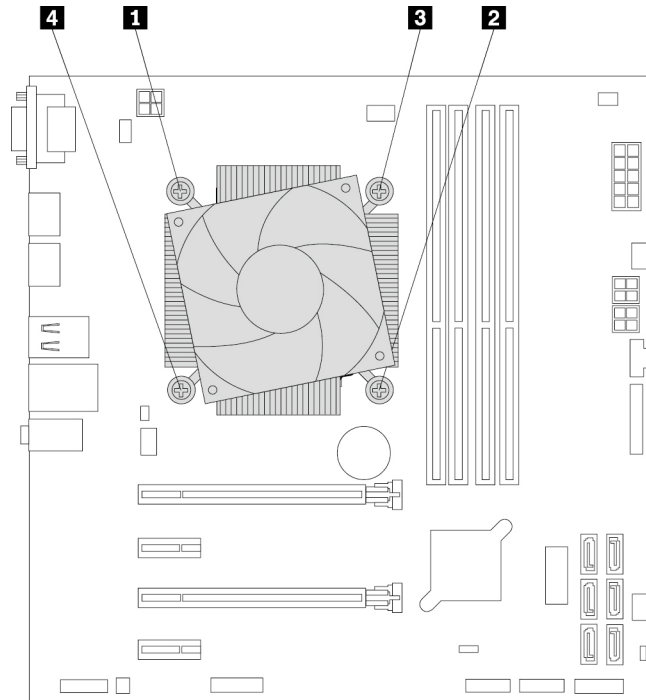
Figure 110. Removing the heat sink and fan assembly
