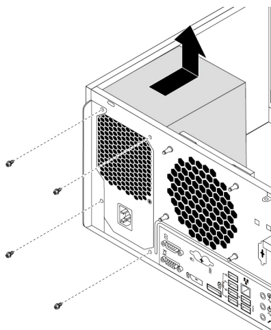
Figure 109. Removing the screws for the power supply assembly
