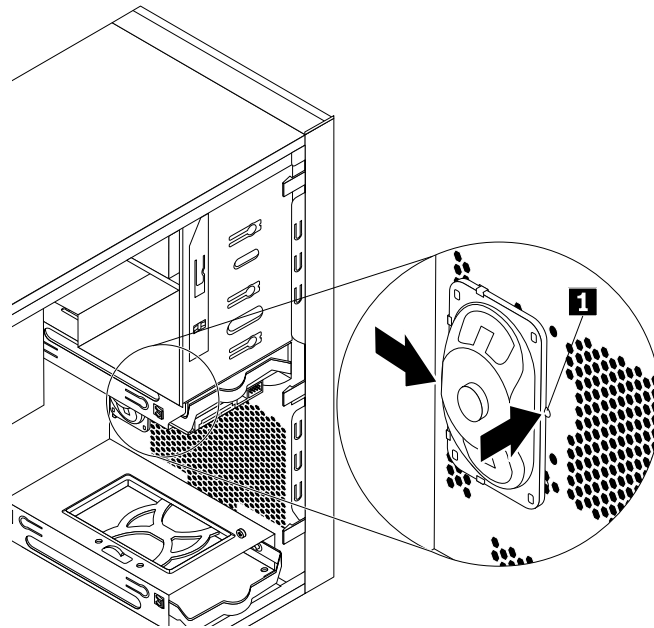
Figure 103. Removing the old internal speaker
